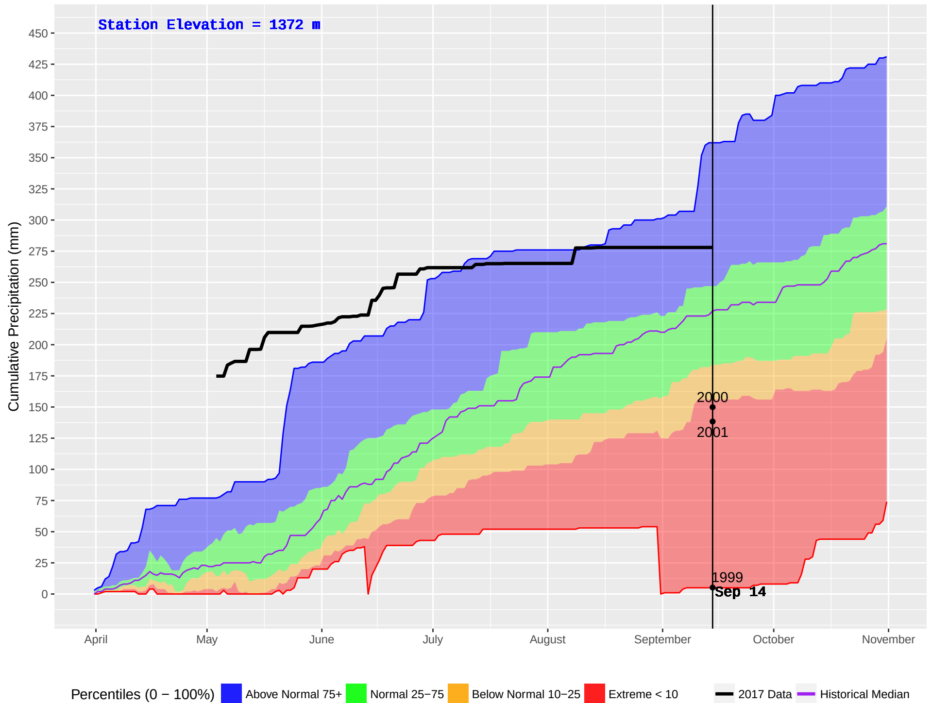
CHERRY LAKE (791) : Historical (1989–2016) and Current (2017) Noon Cumulative Precipitation
