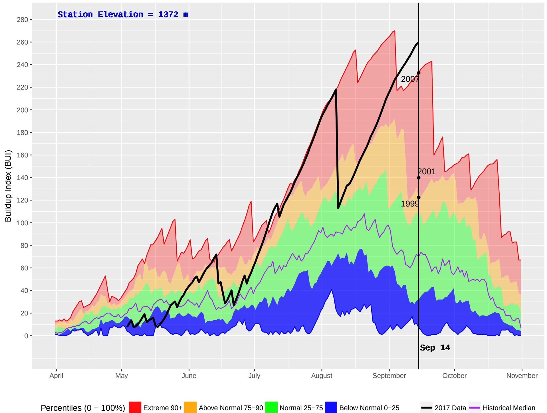
CHERRY LAKE (791) : Historical (1989–2016) and Current (2017) Noon Buildup Index (BUI)
